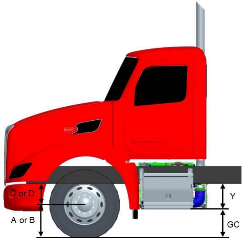
FIGURE 3-26. Ground Clearance Calculations
