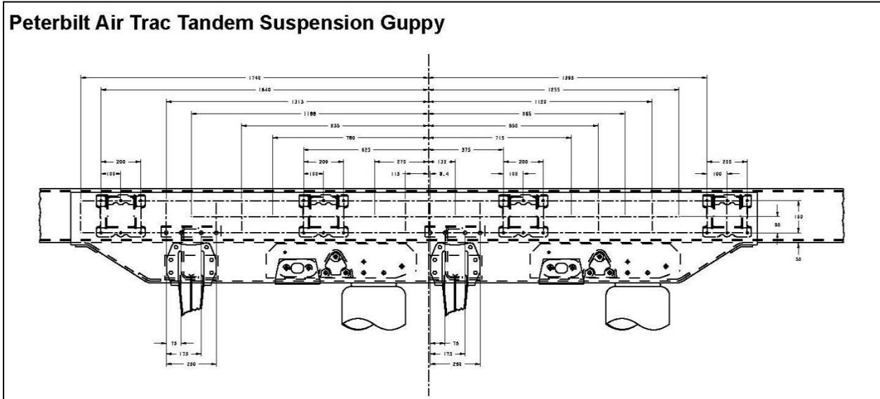
FIGURE 3-18. Peterbilt Air Trac Tandem Suspension Guppy
