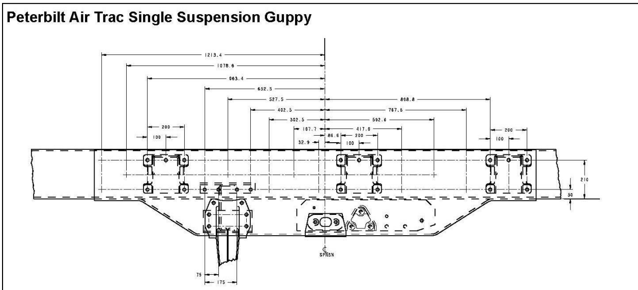
FIGURE 3-19. Peterbilt Air Trac Single Suspension Guppy
