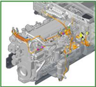
ENGINE HARNESS
