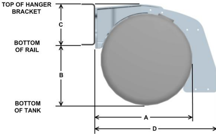
FIGURE 3-28. Fuel Tanks
