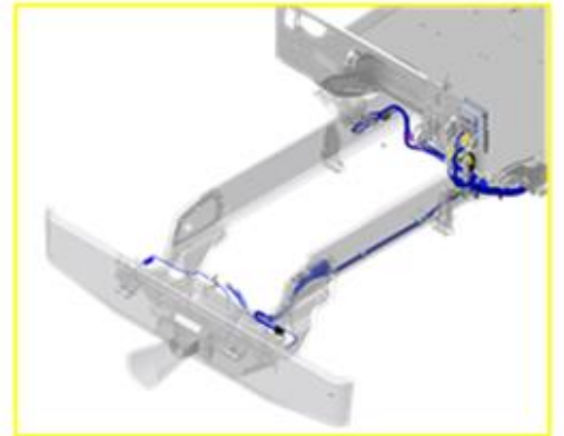
MAIN CHASSIS HARNESS
