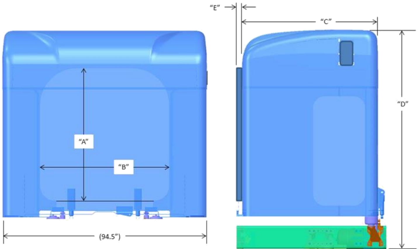
FIGURE 3-10. Sleeper Dimensions – Front & LH View
