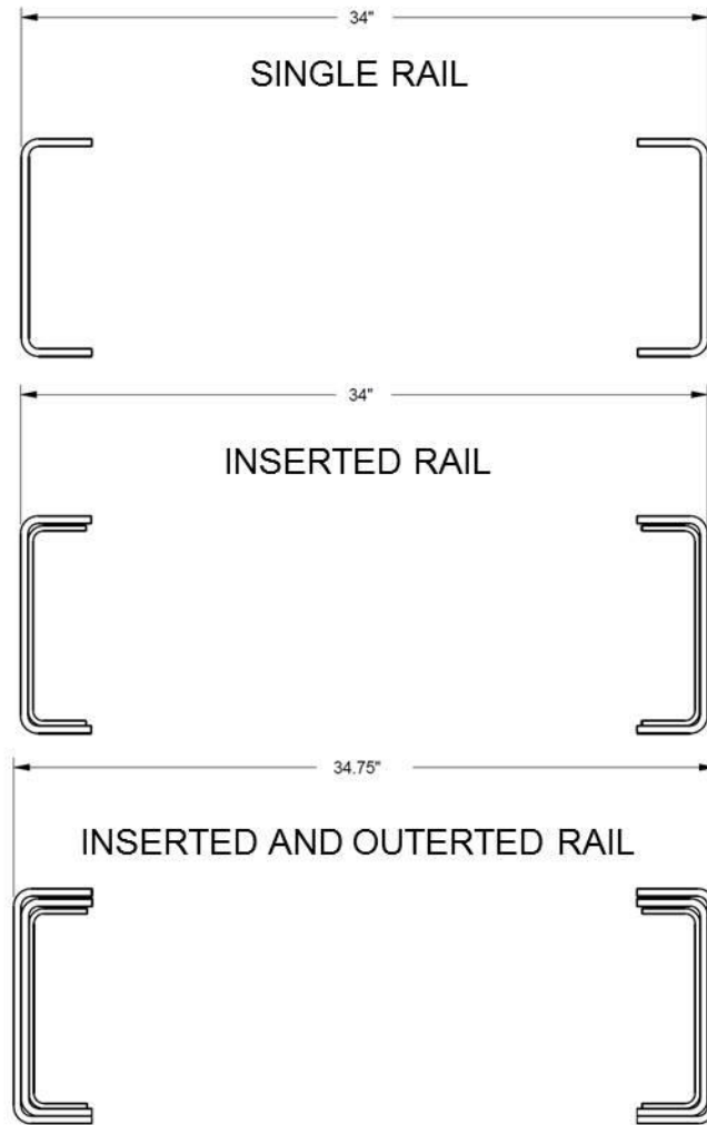
FIGURE 3-11. Frame Rail Configurations
