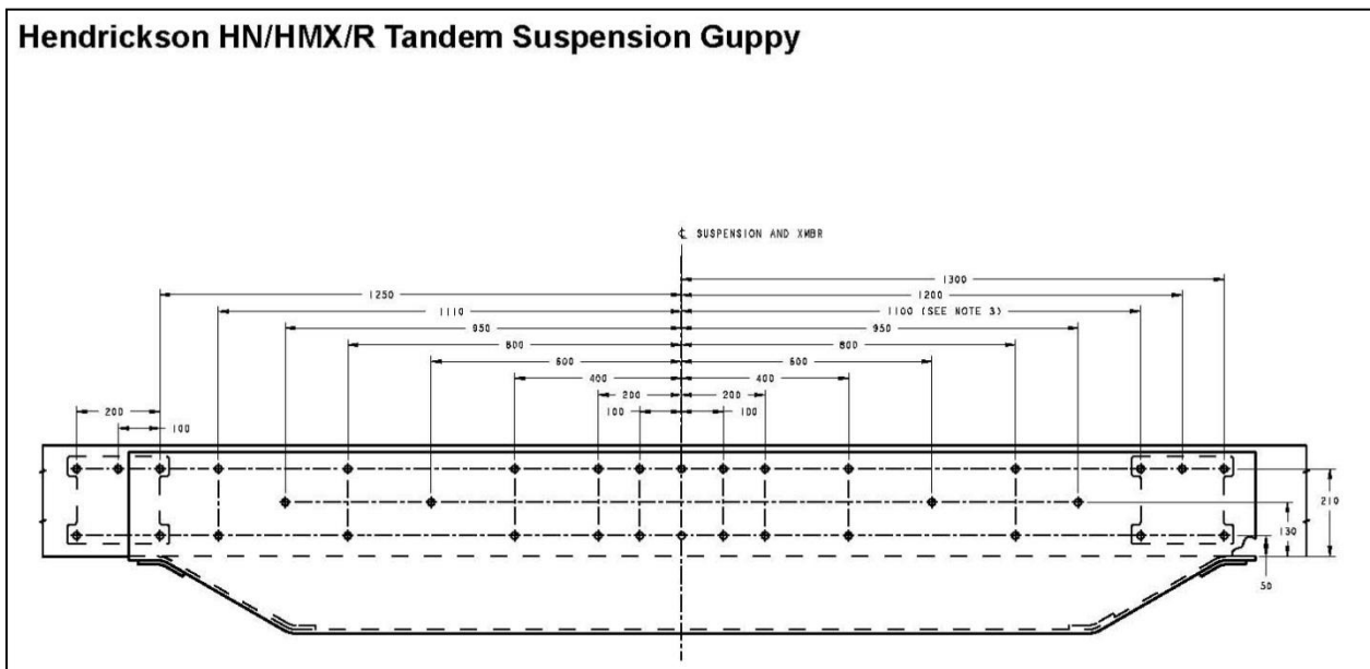
FIGURE 3-21. Hendrickson HN/HMX/R Tandem Suspension Guppy
