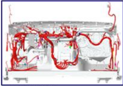
MAIN CAB (IP) HARNESS
