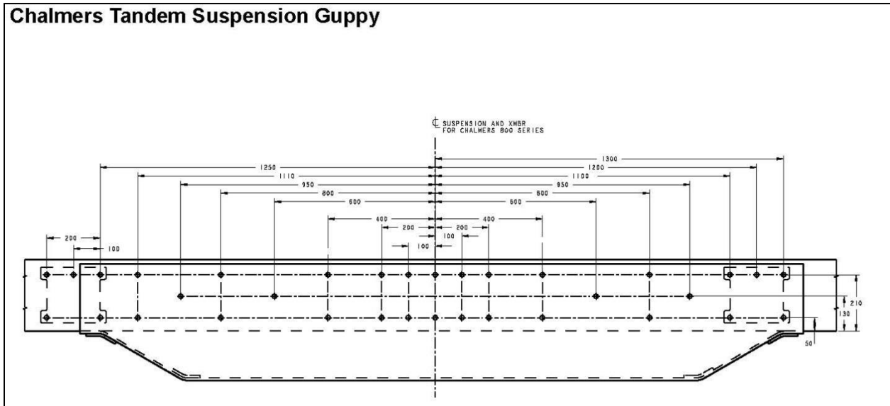
FIGURE 3-20. Chalmers Tandem Suspension Guppy
